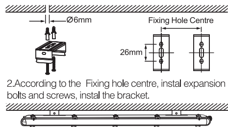
4. Finish installation
